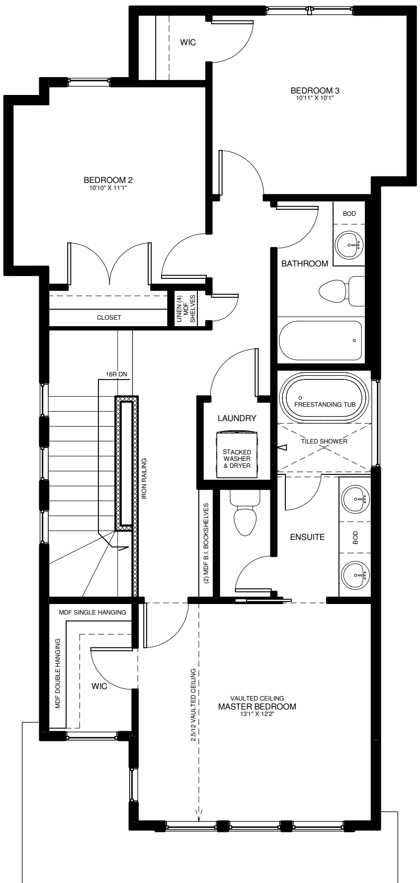
UPPER FLOOR
