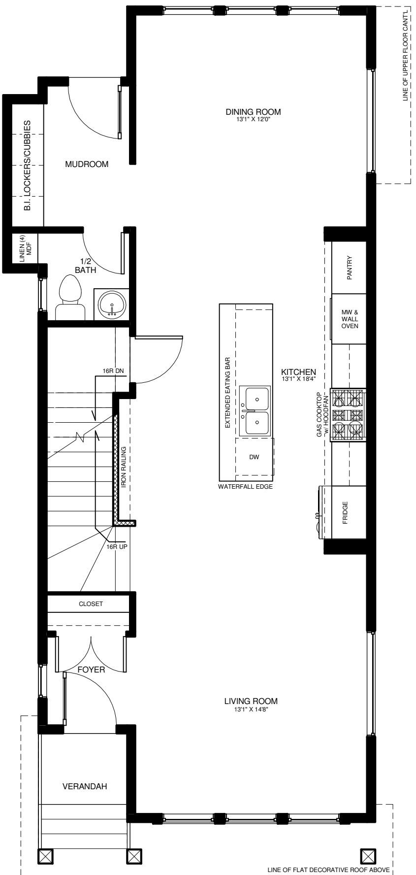
MAIN FLOOR
