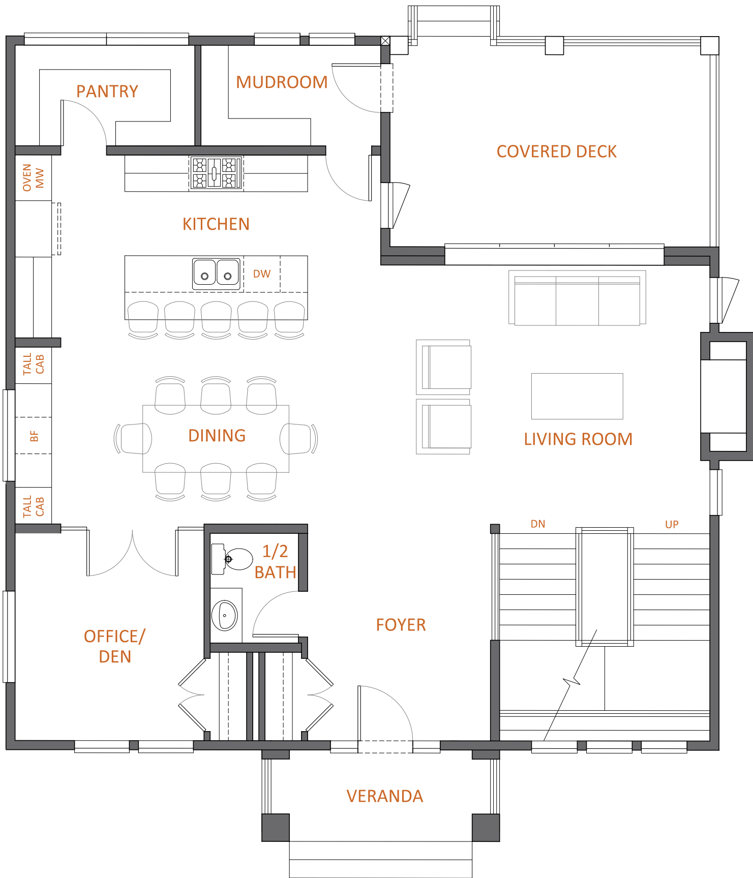
MAIN FLOOR PLAN 1,314 SQUARE FEET
