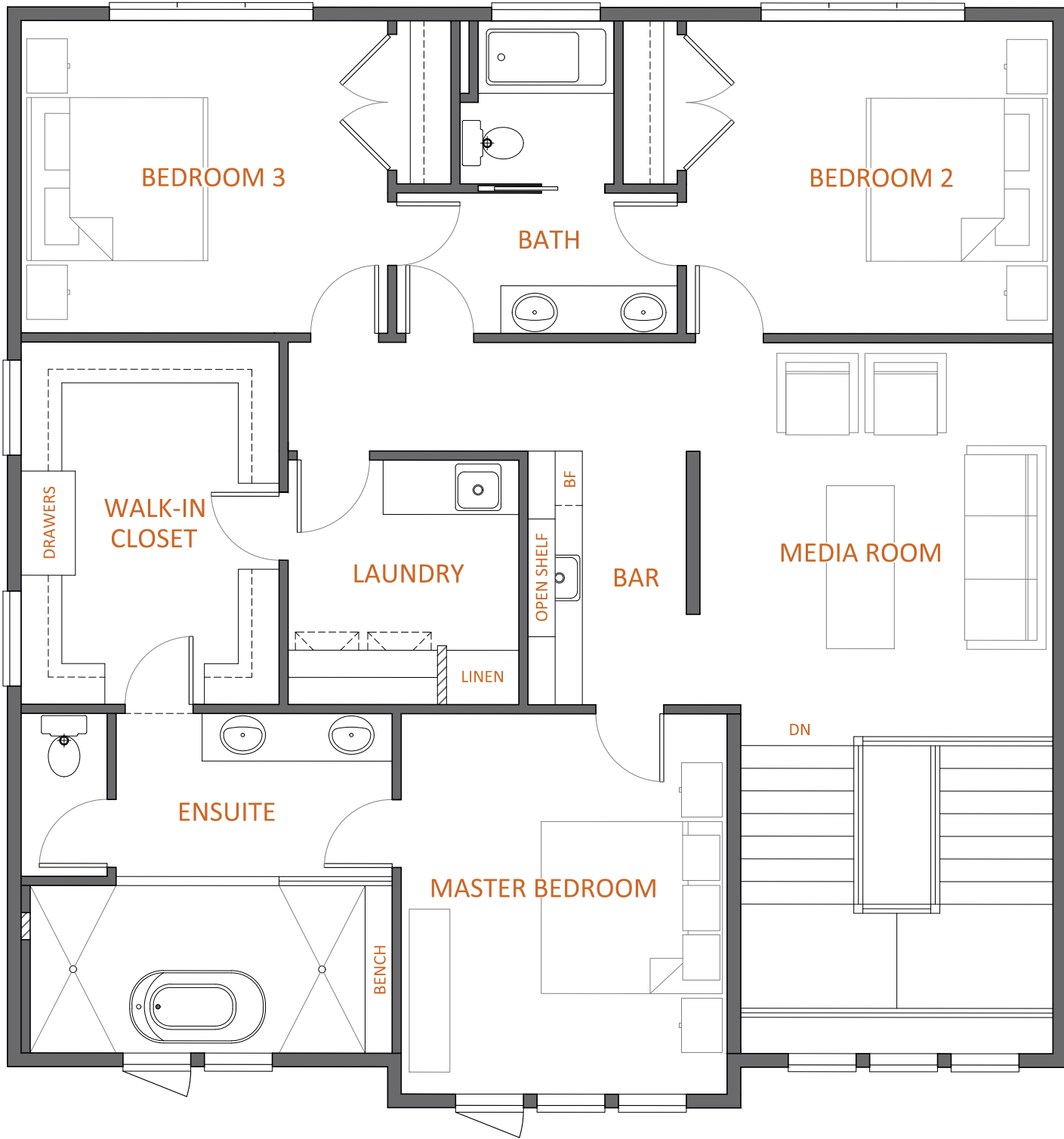
SECOND FLOOR PLAN 1,410 SQUARE FEET
